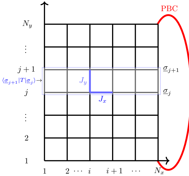
Figure 6.1: The 2-dimensional classical Ising model on a square lattice. The system has N_x \times N_y sites, and PBC are enforced in the y -direction: you can think of the system as “living on a cylinder” with an axis along the x -direction. Boundary conditions along the x -direction are left unspecified: they could be open , fixed , or periodic . In the latter case, you might picture the system as “living on a torus”. The blue lines highlight the couplings J_x , connecting sites (i, j) and (i + 1, j) , and J_y , connecting (i, j) and (i, j + 1) . The shaded rectangle highlights the Boltzmann weights included in the definition of the “transfer matrix” \langle \underline{\sigma}_{j+1} | T | \underline{\sigma}_j \rangle .
