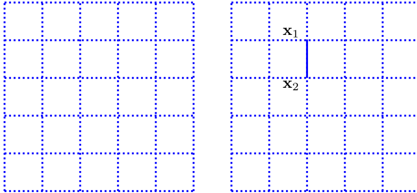
Figure 9.12: Left: The ground state |\Psi_{\text{gs}}\rangle_{h_\perp \rightarrow \infty} with all links in state |+, x\rangle (dotted lines). Right: The lowest-energy excited states where two violations of \hat{G}_{\mathbf{x}} = 1 appear at the vertices denoted as \mathbf{x}_1 and \mathbf{x}_2 , and a single link (the full blue line) is in the state |-, \mathbf{x}\rangle = \hat{\sigma}_\ell^z |+, x\rangle_\ell .
