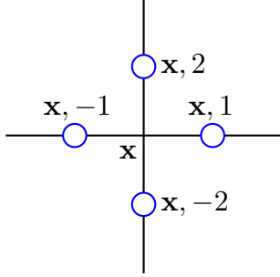
Figure 9.2: An internal vertex at \mathbf{x} and the four neighboring links in a d = 2 dimensional (square) lattice, defining the \text{star}(\mathbf{x}) . The operator \hat{G}_{\mathbf{x}} = \hat{\sigma}_{\mathbf{x},1}^x \hat{\sigma}_{\mathbf{x},2}^x \hat{\sigma}_{\mathbf{x},-1}^x \hat{\sigma}_{\mathbf{x},-2}^x flips the four spins sitting at the blue circles on the links that enter \mathbf{x} .
