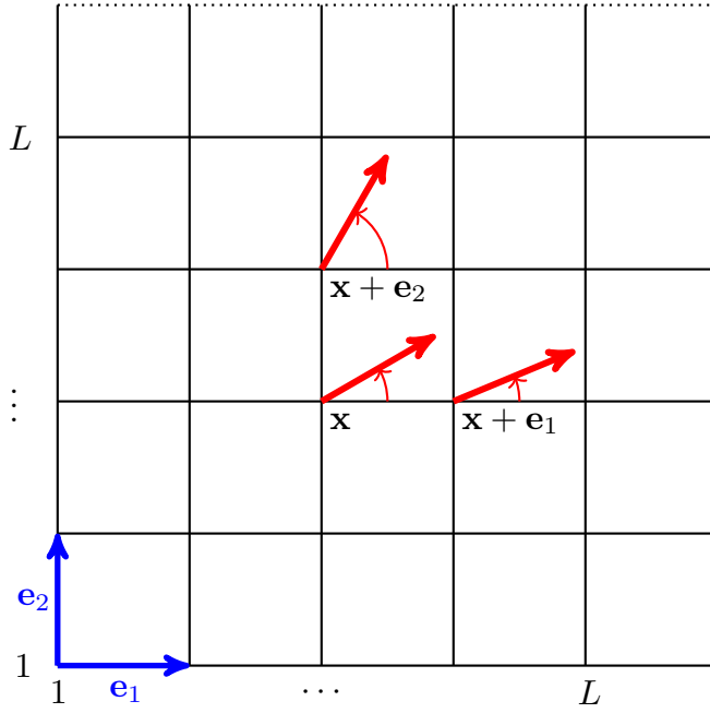
Figure 8.1: The XY model. An L \times L square lattice is shown, with periodic boundary conditions: the dashed borders should be identified with the opposite border, making the geometry that of a torus. The two nearest-neighbor vectors \mathbf{e}_1 and \mathbf{e}_2 are shown in blue. At each lattice site \mathbf{x} a planar spin (classical unit vector on the plane) is uniquely given by the angle \theta_{\mathbf{x}} formed with the x -axis: \mathbf{S}_{\mathbf{x}} = (\cos \theta_{\mathbf{x}}, \sin \theta_{\mathbf{x}}) . Three spins at nearest-neighbor sites \mathbf{x} , \mathbf{x} + \mathbf{e}_1 and \mathbf{x} + \mathbf{e}_2 are shown as thick red arrows (all other spins are omitted for clarity).
