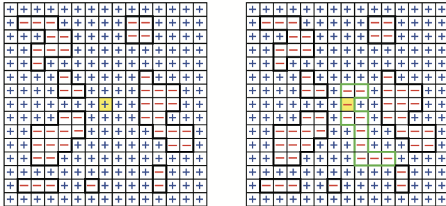
Figure 5.6: The Peierls’ argument to show that the two-dimensional Ising model has a robust broken-symmetry phase surviving at finite T < T_c . The figure, taken from Arovas, poses the problem of how to estimate the difference in probability for the central spin being \uparrow = + with respect to being \downarrow = - , in a large system with boundary conditions set to + , a device alternative to the small longitudinal field trick to test for broken symmetry.
