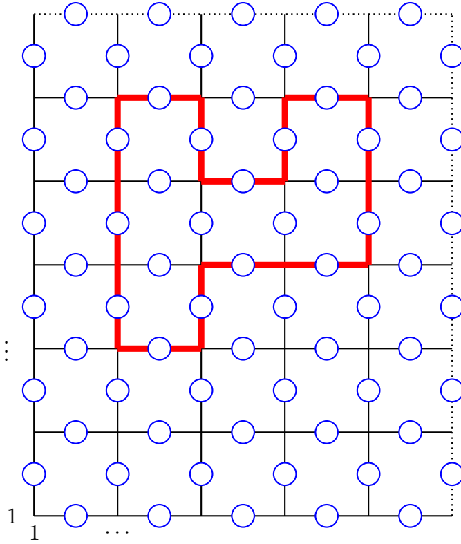
Figure 9.5: The Wilson loop. The closed contour \mathcal{C} (red thick line) contains links \ell and the Wilson loop operator is defined by \hat{Z}_{\mathcal{C}} = \prod_{\ell \in \mathcal{C}} \hat{\sigma}_{\ell}^z . Equivalently, \hat{Z}_{\mathcal{C}} can be seen as the product of all \hat{Z}_{\mathbf{x}_*} plaquette operators where \mathbf{x}_* is inside the contour \mathcal{C} . Here the area inside the loop is A_{\mathcal{C}} = 6 , while its perimeter is P_{\mathcal{C}} = 14 . Notice, however, that the generic situation for large loops is precisely opposite, with A_{\mathcal{C}} > P_{\mathcal{C}} .
