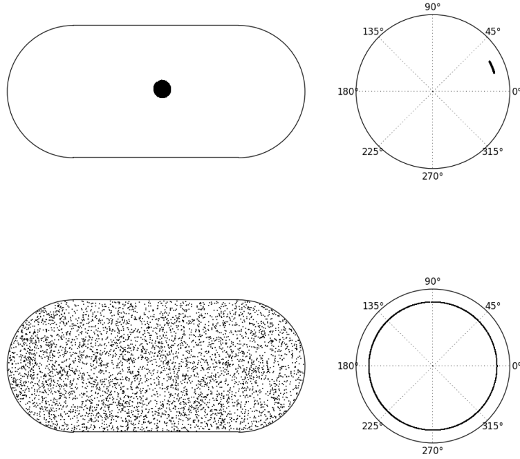
Figure 1.6.: The stadium mixing. (Top) The initial conditions, with configurations on the left and velocities on the right. (Bottom) A snapshot at a sufficiently large time. Figures due to Simone Ziraldo.
