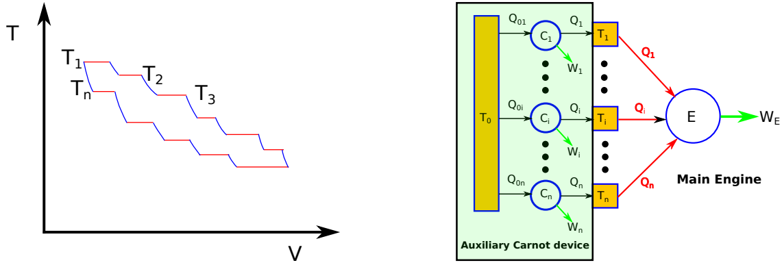
Figure 2.3.: Left: A cycle in the T - V plane working with n reservoirs at temperatures T_i . Red horizontal lines are isotherms (with an exchange of heat Q_i ), blue lines are adiabats (just a sketch) during which no heat is exchanged. Right: An arbitrary engine E exchanging heat Q_i during isotherms with reservoirs at temperatures T_i , producing a work W_E^{\text{ext}} . The left part sketches the auxiliary system made by n Carnot reversible engines so devised that they “give back” (if Q_i > 0 ) or “take” (if Q_i < 0 ) exactly an amount of heat Q_i from each T_i -reservoir, while their second reservoir is a common one at temperature T_0 .
