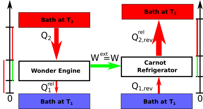
Figure 2.2.: The set-up to prove Carnot’s theorem. The width of the arrows indicates the amount of heat. The green and red segments on the left and right axis correspond to the work and heat. The efficiency is the ratio of “green to red segments”: the lower is the position of the rectangle denoting the system, the larger is the efficiency. The supposed larger efficiency for the wonder engine implies less released heat (smaller arrow, lower system box) as compared to the heat absorbed by the Carnot refrigerator, using the same work extracted from the wonder engine. The net result is heat transferred from T_1 to T_2 , against Clausius’ formulation of the 2nd law.
